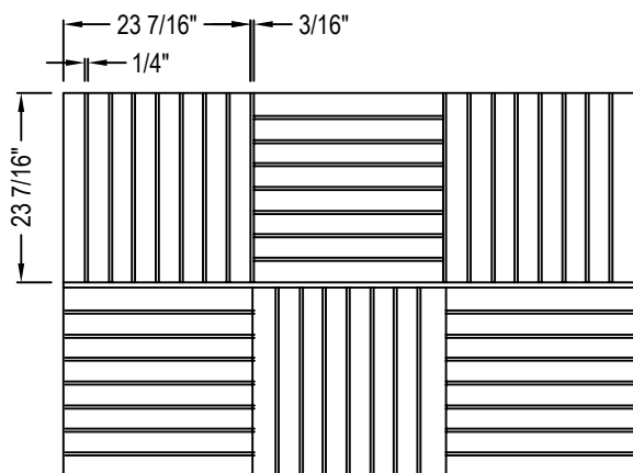
TOP VIEW 23 7/16" X 23 7/16" TILE
