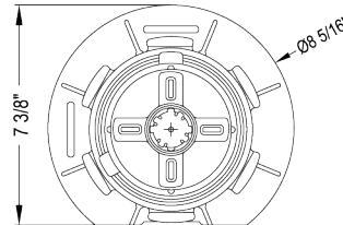
PLAN VIEW PR2
