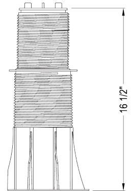
ELEVATION VIEW PR3 (MAXIMUM HEIGHT)
