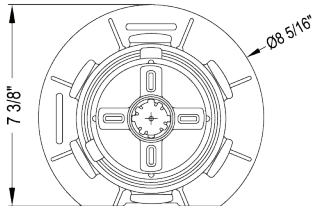
PLAN VIEW PRO
