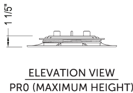
DETAIL PPR EXTENSION
