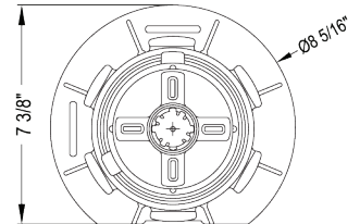
PLAN VIEW PR3
