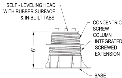
ELEVATION VIEW PR2 (MAXIMUM HEIGHT)
