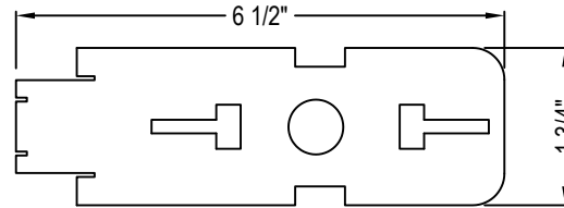
TOP VIEW UPPER CLOSURE CLIP
