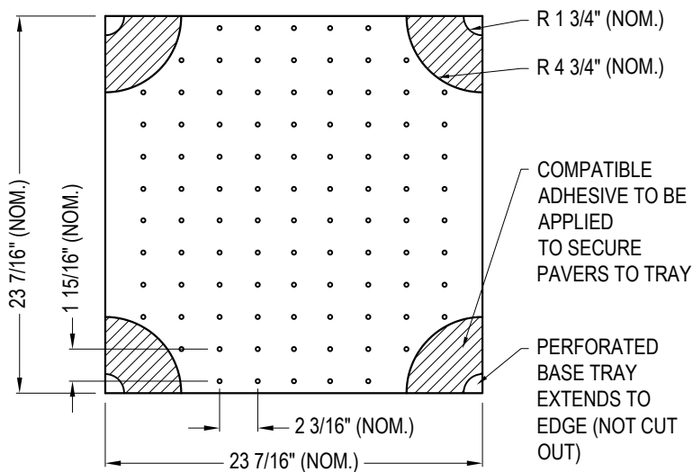
PLAN VIEW ARCHATRAK STEEL TRAY
