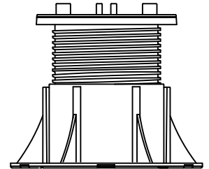
DETAIL NM4: 3 1/2" - 6 1/4"
