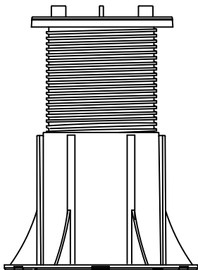
DETAIL NM5: 5 7/8" - 10 5/8"
