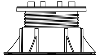
DETAIL NM3: 2 1/4" - 3 7/8"
