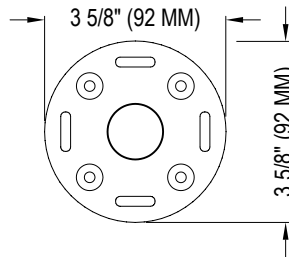
SIDE VIEW PEDESTAL HEAD
