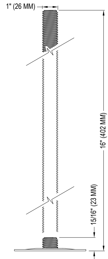
SIDE VIEW BASE
