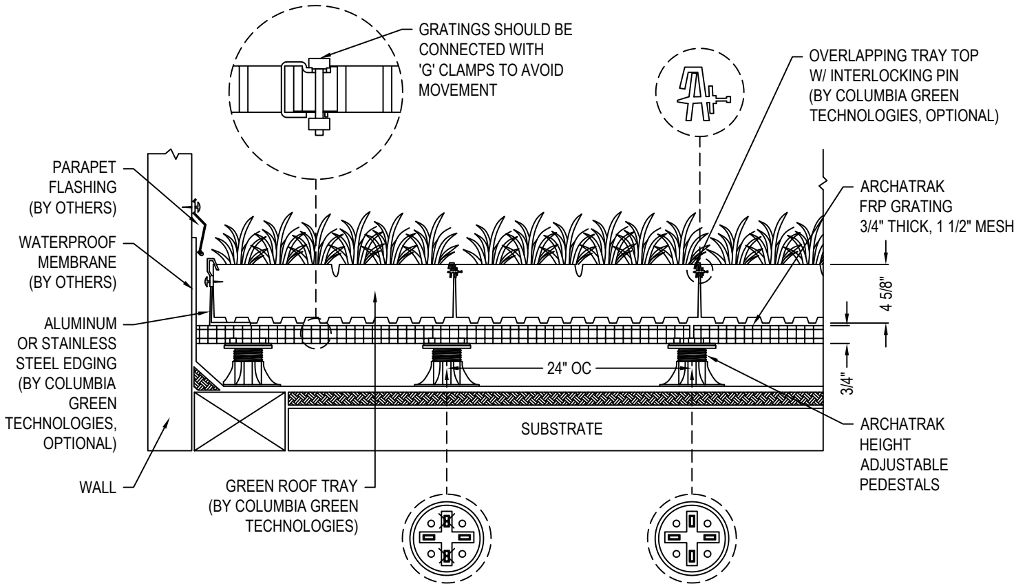
SECTION VIEW
