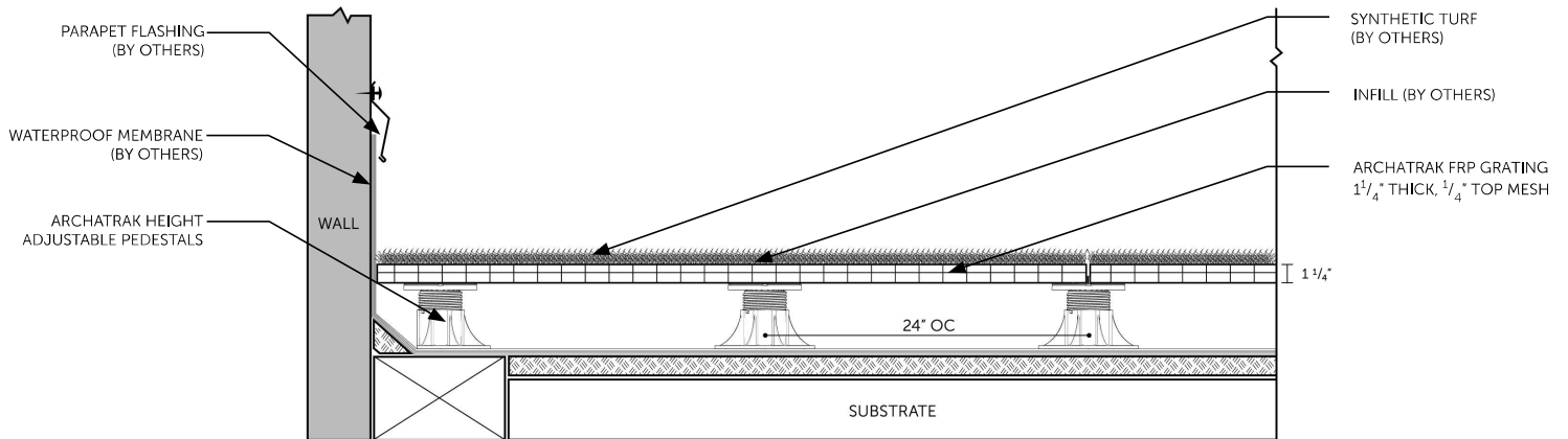
SECTION VIEW
