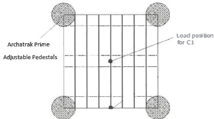
Figure 1. Point Load Test Setup
