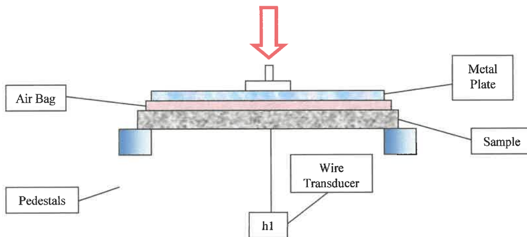
Figure 2. Uniform Load Test Setup
