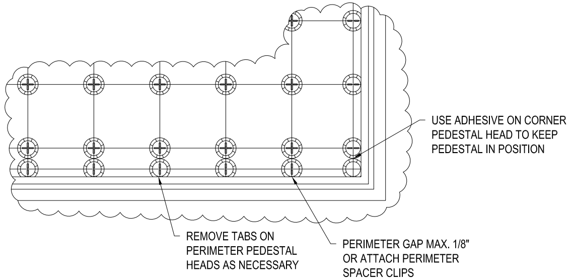
PLAN VIEW
