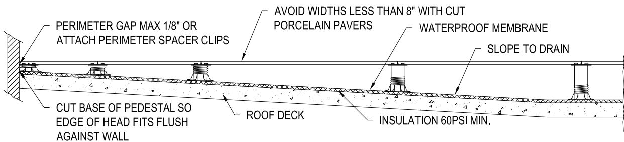
SECTION VIEW
