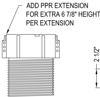
DETAIL PPR EXTENSION
