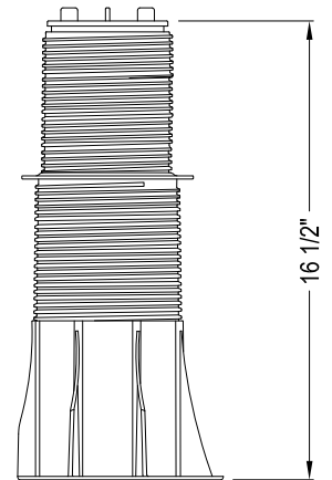
ELEVATION VIEW PR3 (MAXIMUM HEIGHT)
