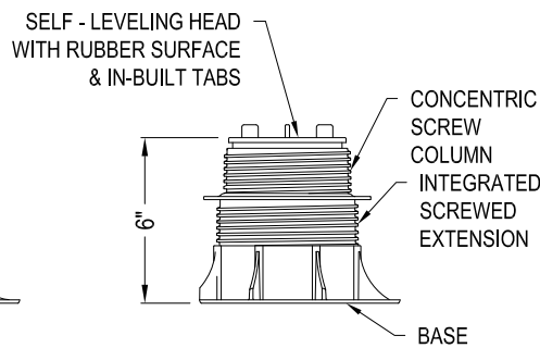
ELEVATION VIEW PR2 (MAXIMUM HEIGHT)
