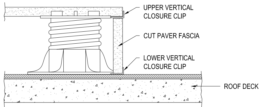
SECTION VIEW
