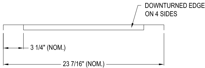
PLAN VIEW BREAK THROUGH PROTECTION PLATE GALVANIZED STEEL
