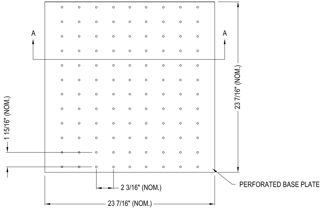
PLAN VIEW BREAK THROUGH PROTECTION PLATE GALVANIZED STEEL
