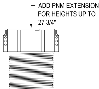
DETAIL EXT: 6 1/2"
