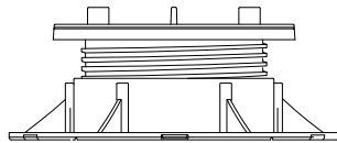
DETAIL NM2: 1 5/8" - 2 1/4"
