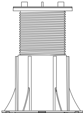
DETAIL NM5: 5 7/8" - 10 5/8"
