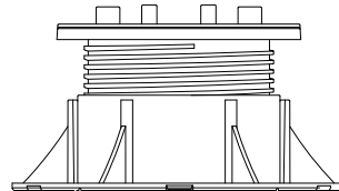
DETAIL NM3: 2 1/4" - 3 7/8"
