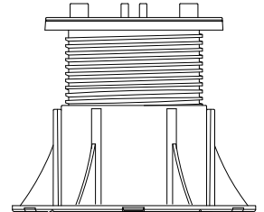
DETAIL NM4: 3 1/2" - 6 1/4"
