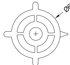
DETAIL TW-150: SLOPE COMPENSATION RINGS 1/16" - 1/8"
